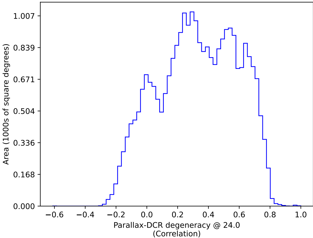
baseline_v3.4_10yrs : Parallax-DCR degeneracy @ 24.0
