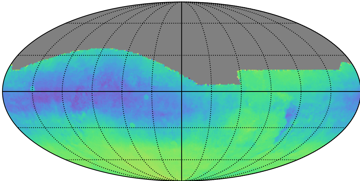
baseline_v3.4_10yrs : Parallax-DCR degeneracy @ 22.4
