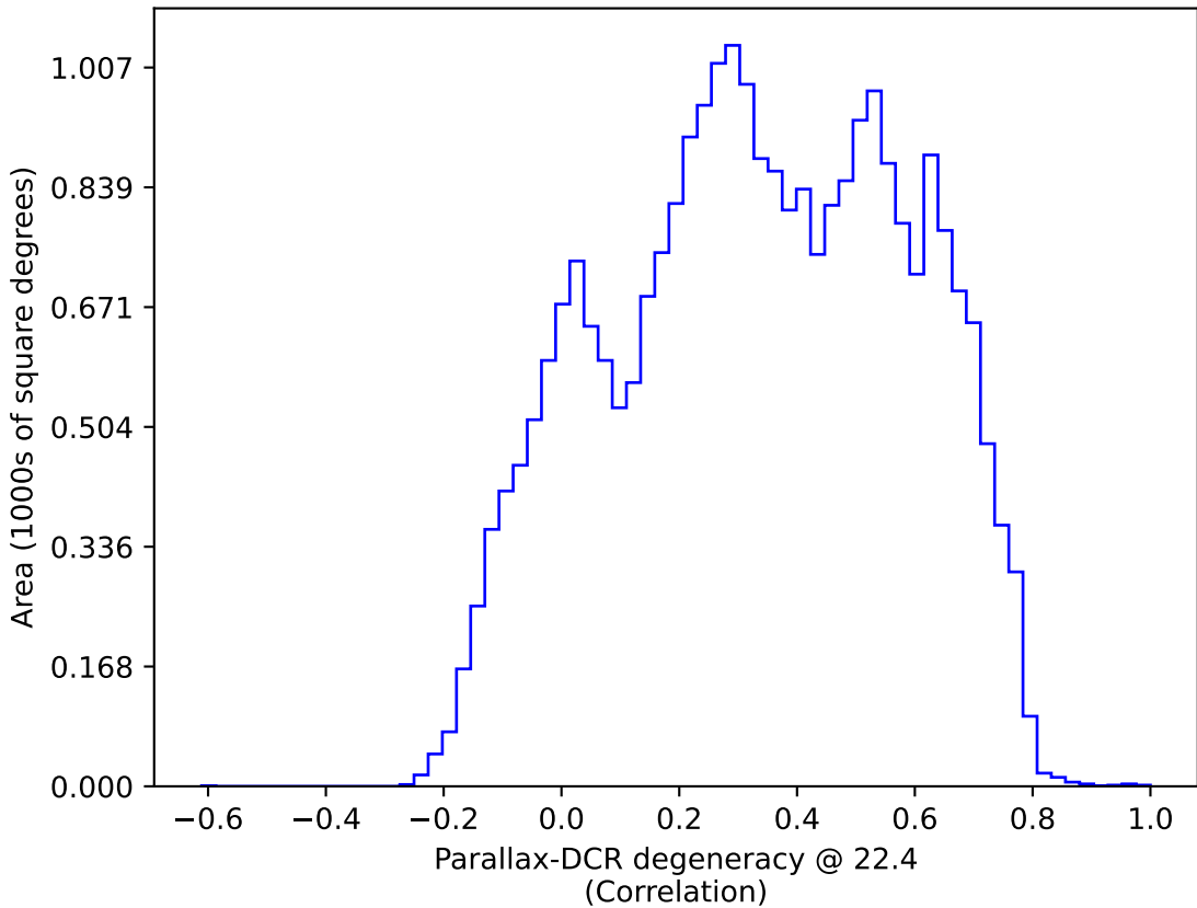
baseline_v3.4_10yrs : Parallax-DCR degeneracy @ 22.4
