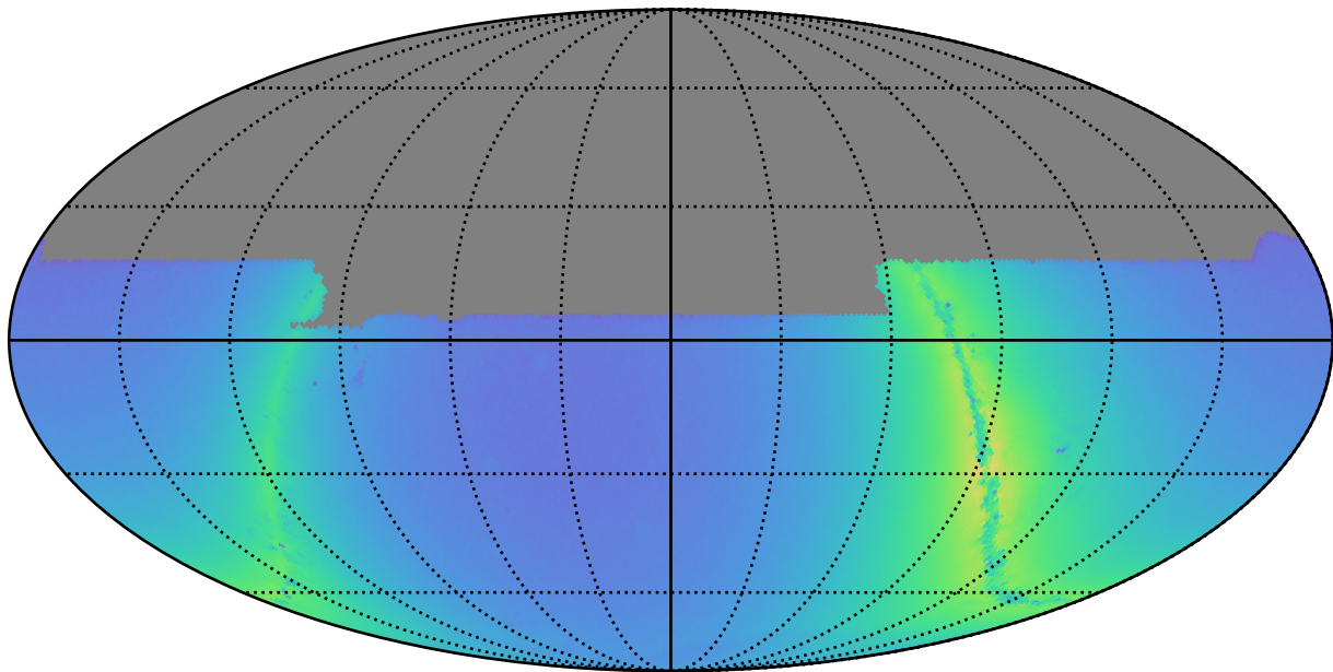
baseline_v3.4_10yrs y: Nstars_no_crowding
