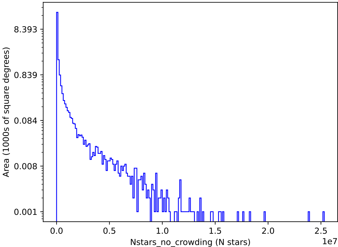
baseline_v3.4_10yrs y: Nstars_no_crowding
