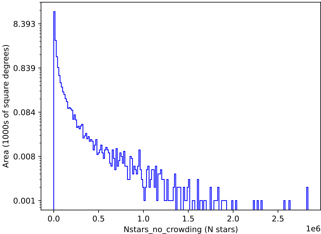
baseline_v3.4_10yrs u: Nstars_no_crowding
