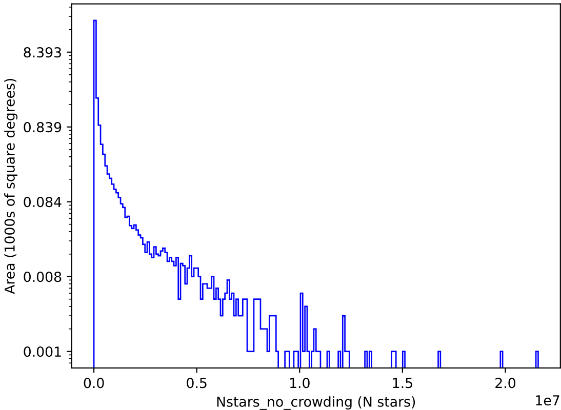
baseline_v3.4_10yrs r: Nstars_no_crowding
