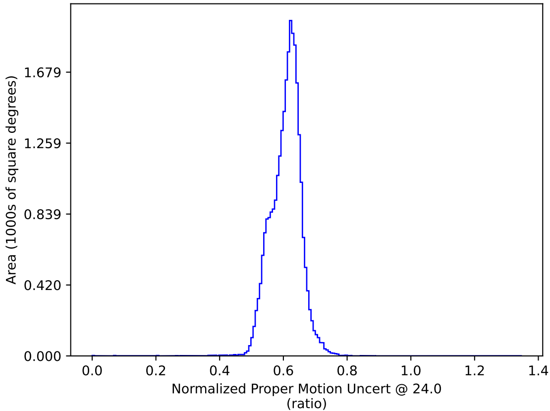
baseline_v3.4_10yrs : Normalized Proper Motion Uncert @ 24.0
