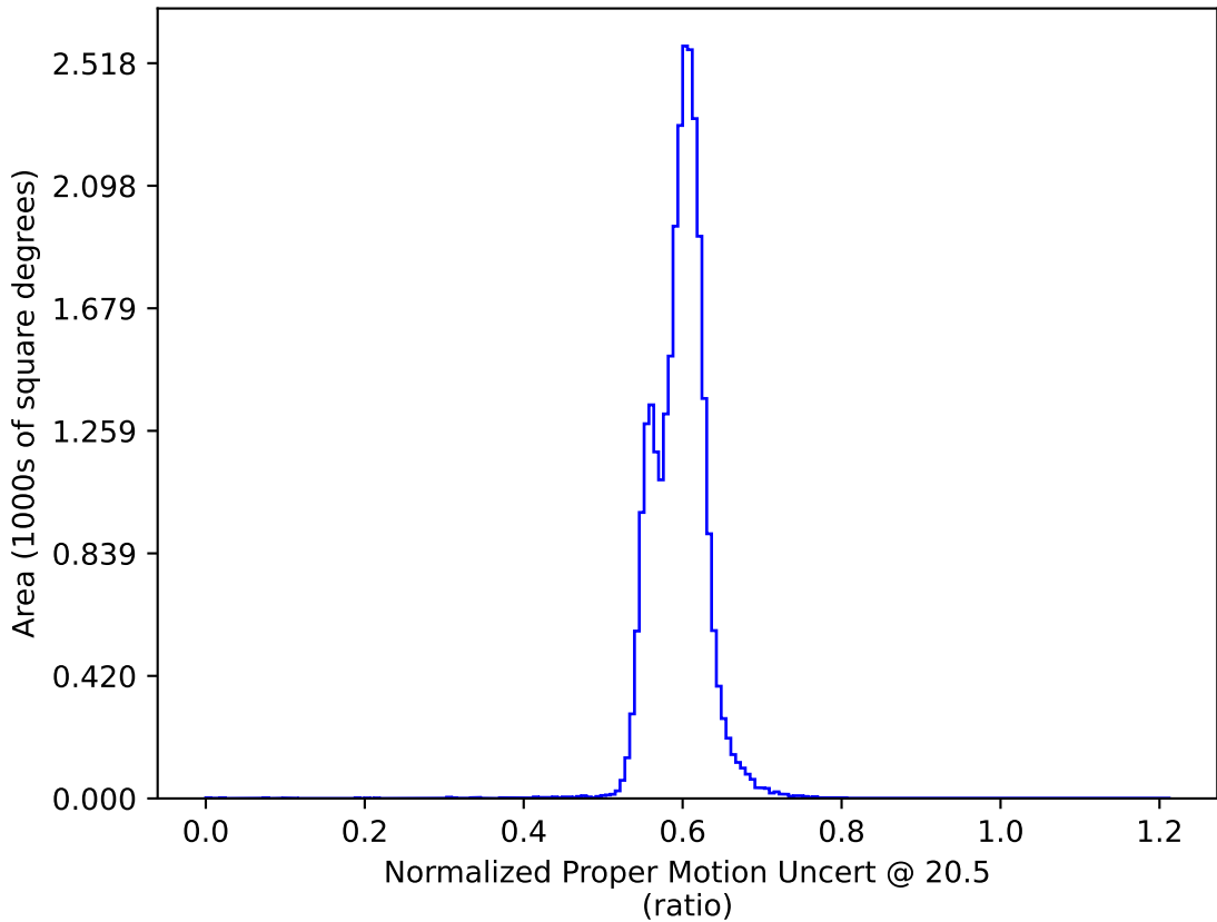
baseline_v3.4_10yrs : Normalized Proper Motion Uncert @ 20.5
