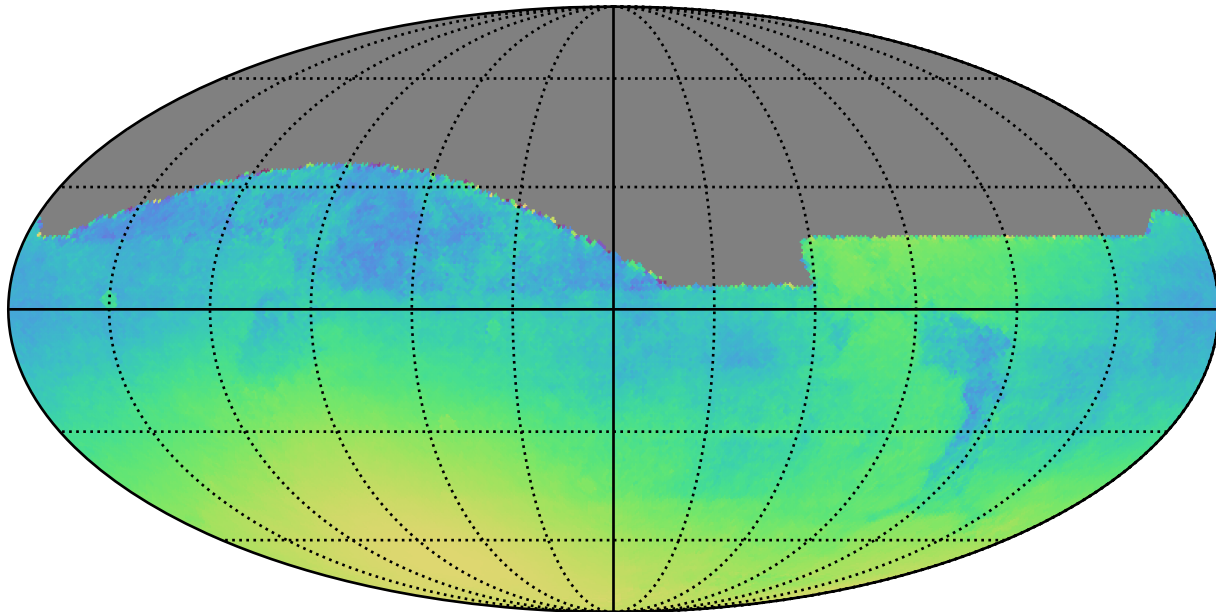
baseline_v3.4_10yrs : Normalized Parallax Uncert @ 24.0
