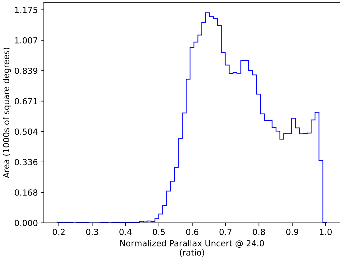
baseline_v3.4_10yrs : Normalized Parallax Uncert @ 24.0
