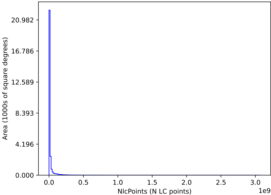
baseline_v3.4_10yrs : NlcPoints
