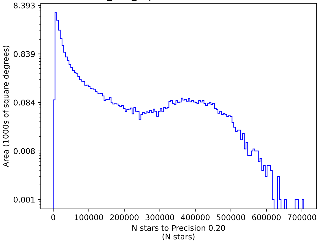
baseline_v3.4_10yrs z: N stars to Precision 0.20
