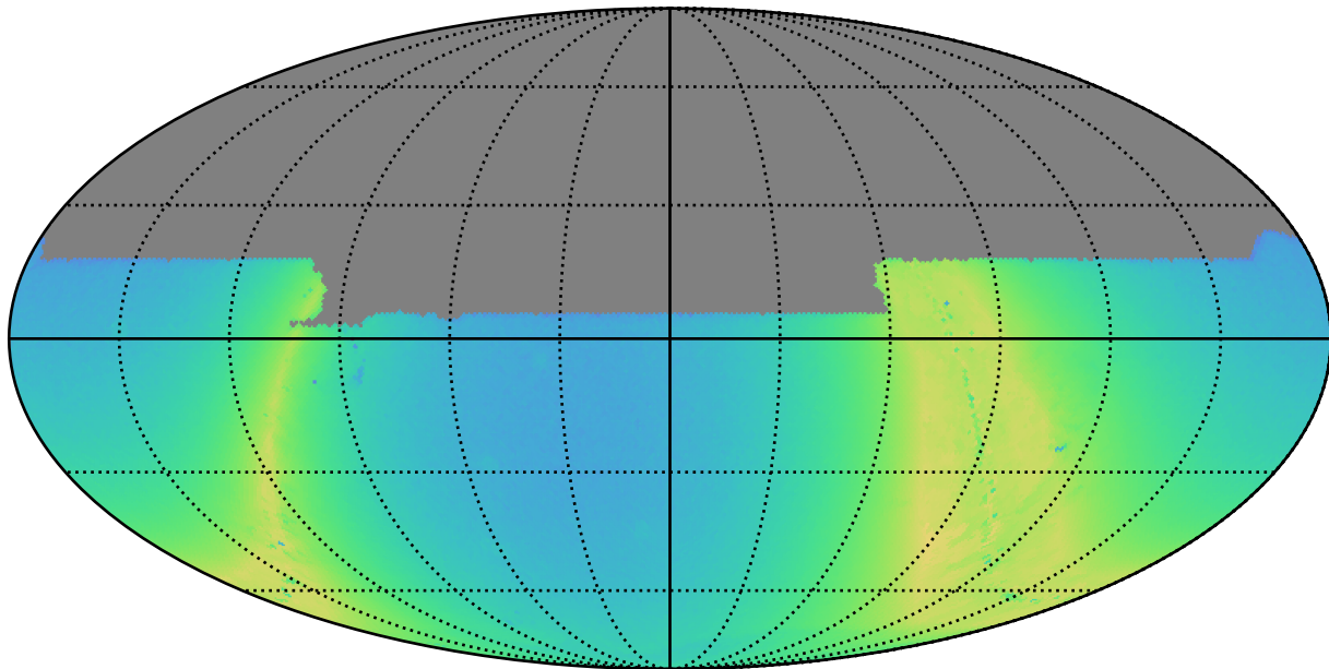
baseline_v3.4_10yrs y: N stars to Precision 0.20
