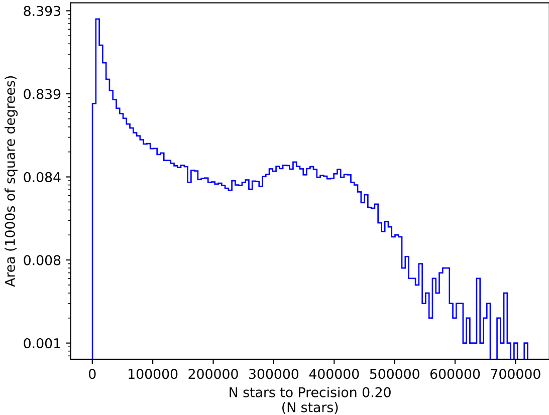
baseline_v3.4_10yrs y: N stars to Precision 0.20
