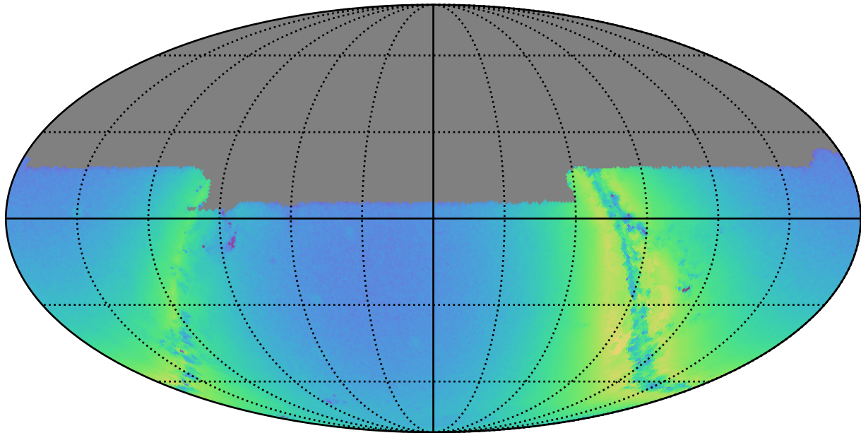
baseline_v3.4_10yrs u: N stars to Precision 0.20
