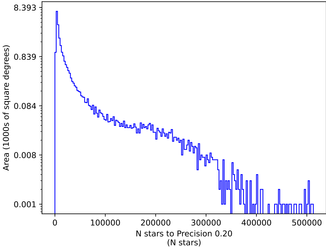
baseline_v3.4_10yrs u: N stars to Precision 0.20
