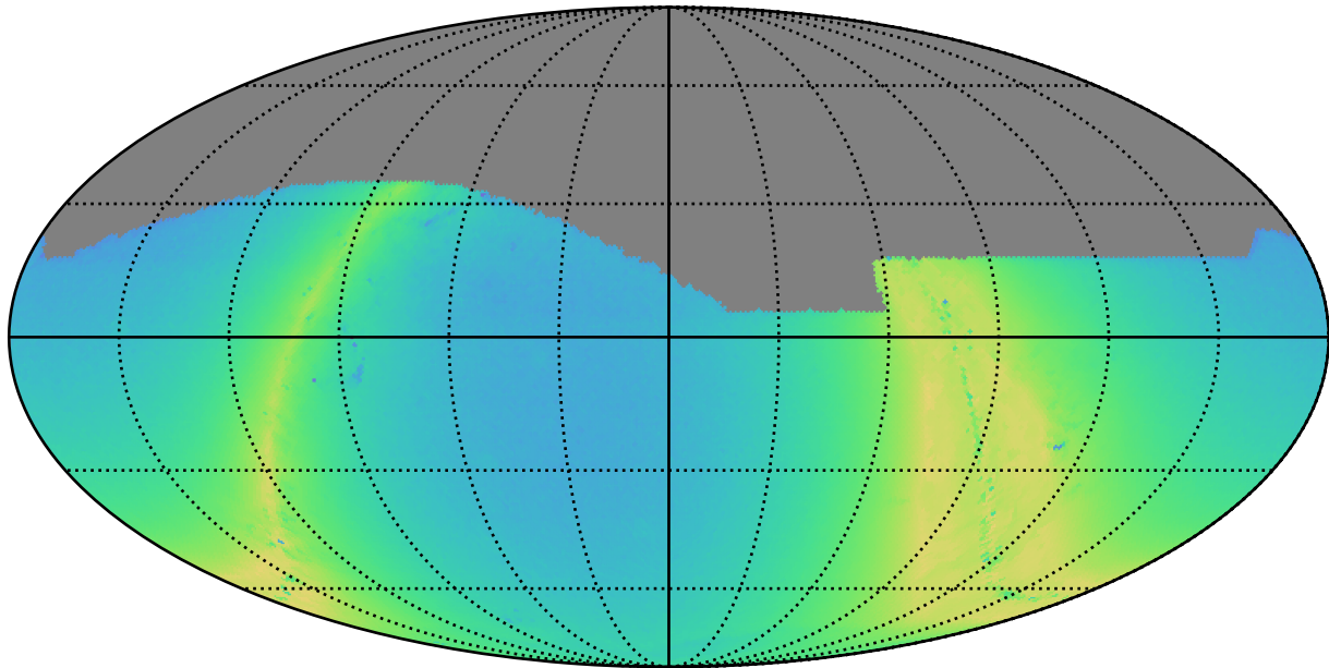
baseline_v3.4_10yrs r: N stars to Precision 0.20
