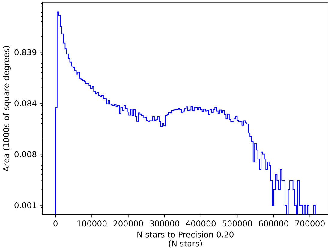
baseline_v3.4_10yrs r: N stars to Precision 0.20
