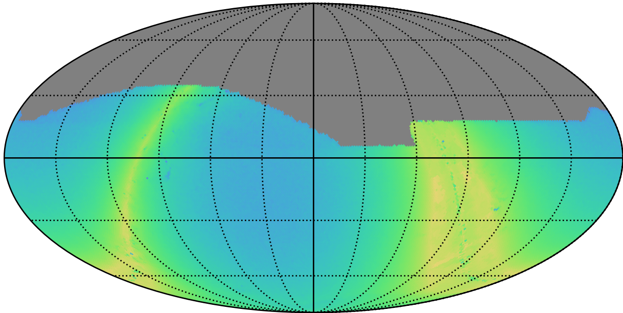
baseline_v3.4_10yrs i: N stars to Precision 0.20
