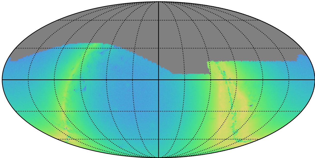
baseline_v3.4_10yrs g: N stars to Precision 0.20
