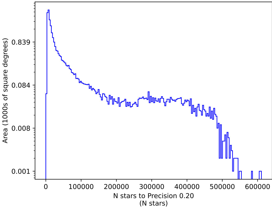
baseline_v3.4_10yrs g: N stars to Precision 0.20
