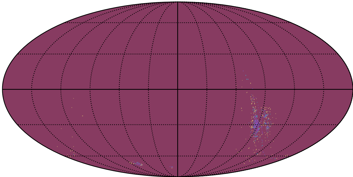
baseline_v3.4_10yrs tE 5_10 days: MicrolensingMetric_detect
