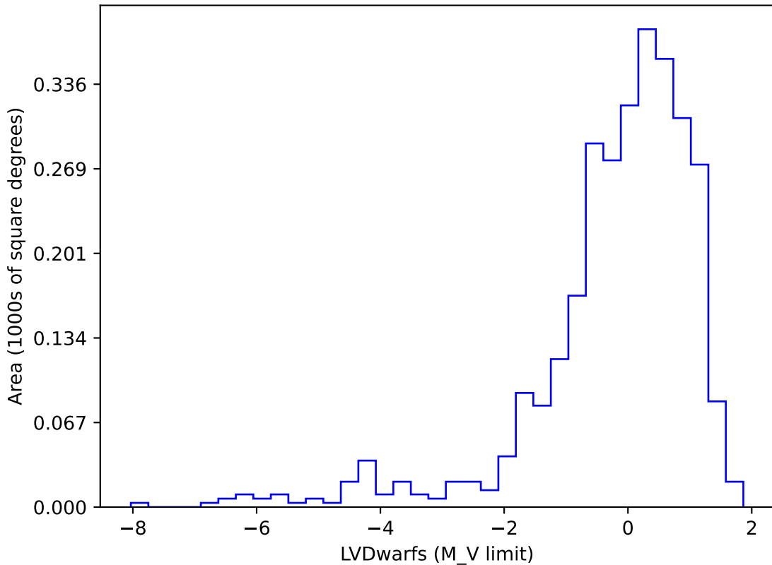
baseline_v3.4_10yrs gi SCP: LVDwarfs
