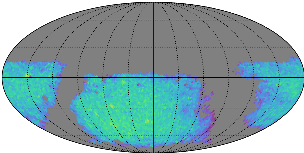
baseline_v3.4_10yrs gi: LVDwarfs
