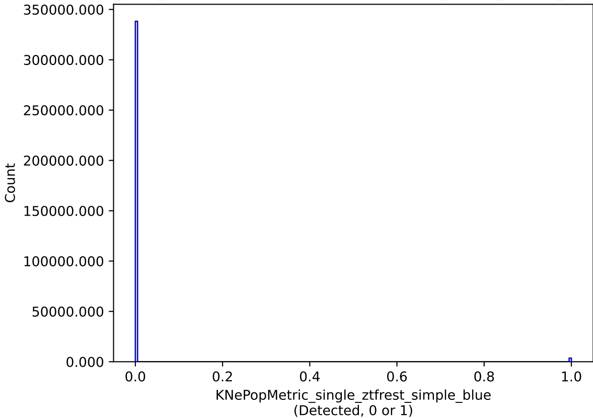
baseline_v3.4_10yrs single model: KNePopMetric_single_ztfrest_simple_blue
