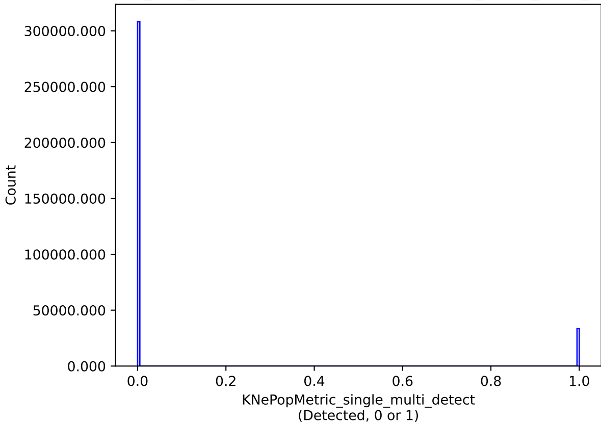
baseline_v3.4_10yrs single model: KNePopMetric_single_multi_detect
