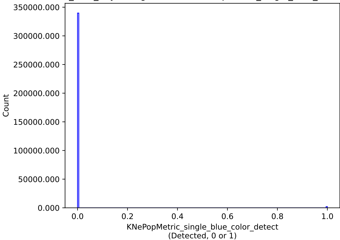
baseline_v3.4_10yrs single model: KNePopMetric_single_blue_color_detect
