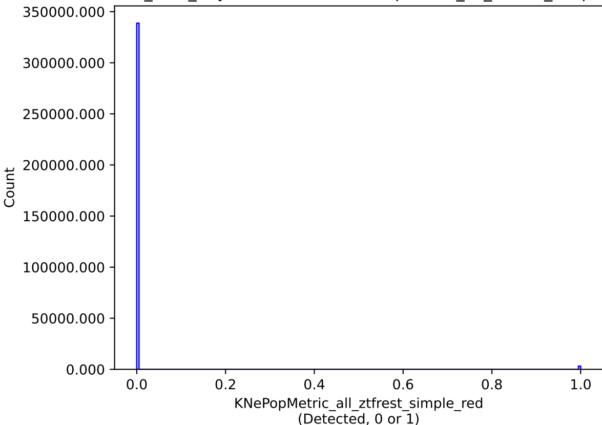
baseline_v3.4_10yrs all models: KNePopMetric_all_ztfrest_simple_red
