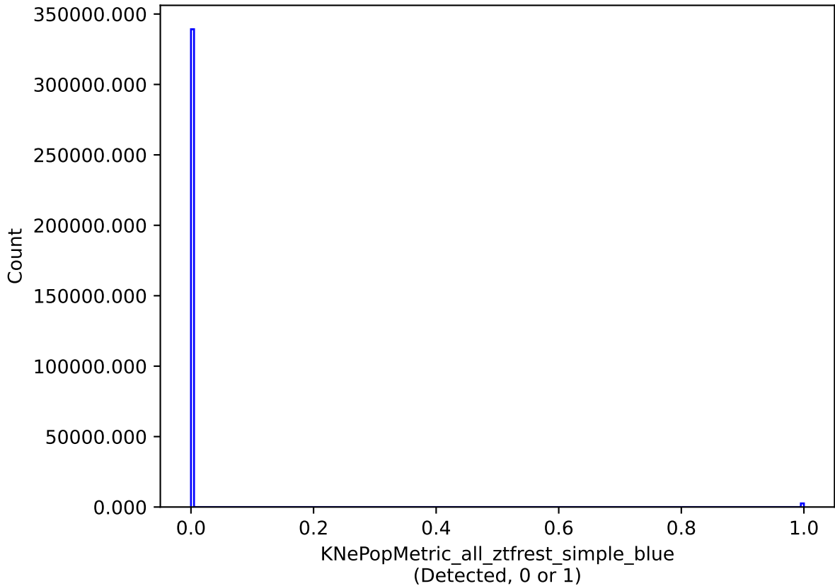
baseline_v3.4_10yrs all models: KNePopMetric_all_ztfrest_simple_blue
