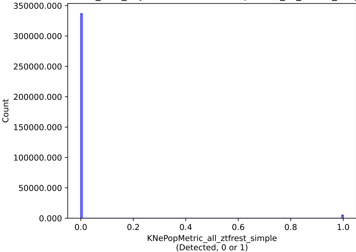
baseline_v3.4_10yrs all models: KNePopMetric_all_ztfrest_simple
