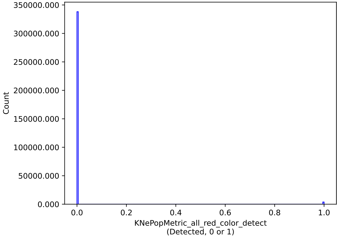
baseline_v3.4_10yrs all models: KNePopMetric_all_red_color_detect
