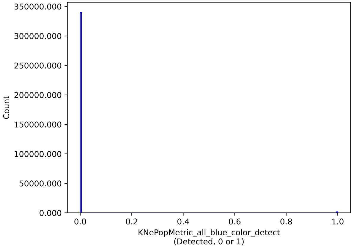
baseline_v3.4_10yrs all models: KNePopMetric_all_blue_color_detect
