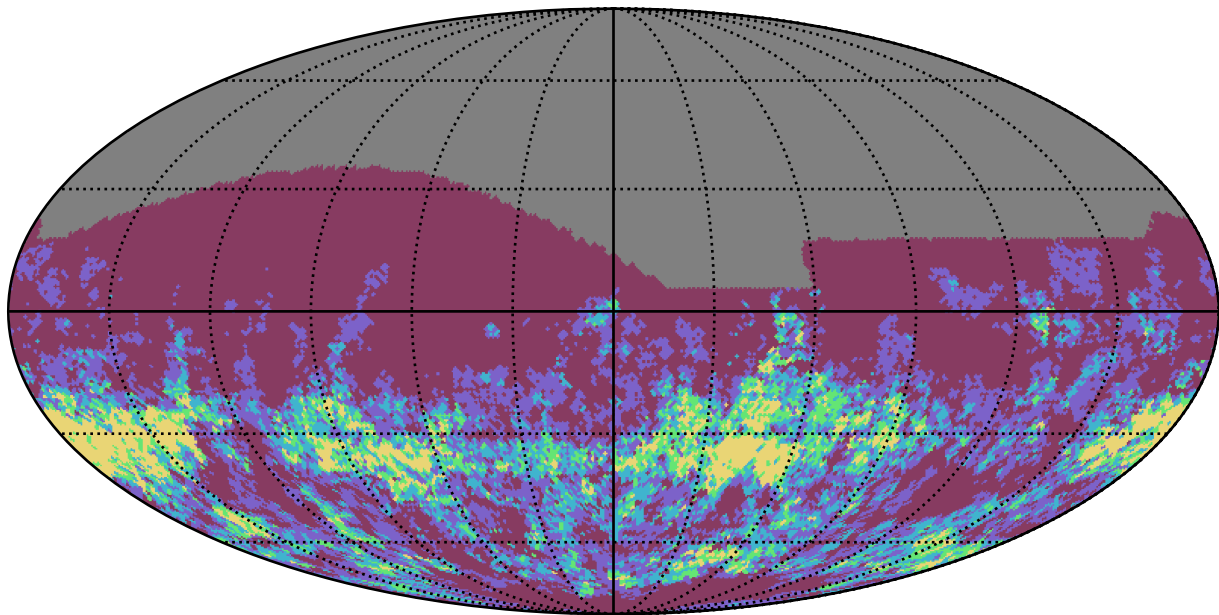
baseline_v3.4_10yrs r band: Gaps_7hr
