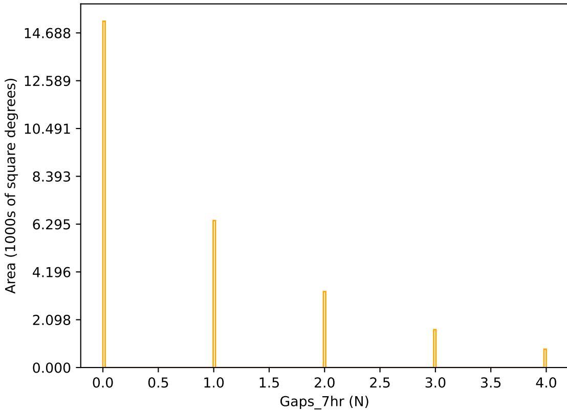
baseline_v3.4_10yrs r band: Gaps_7hr
