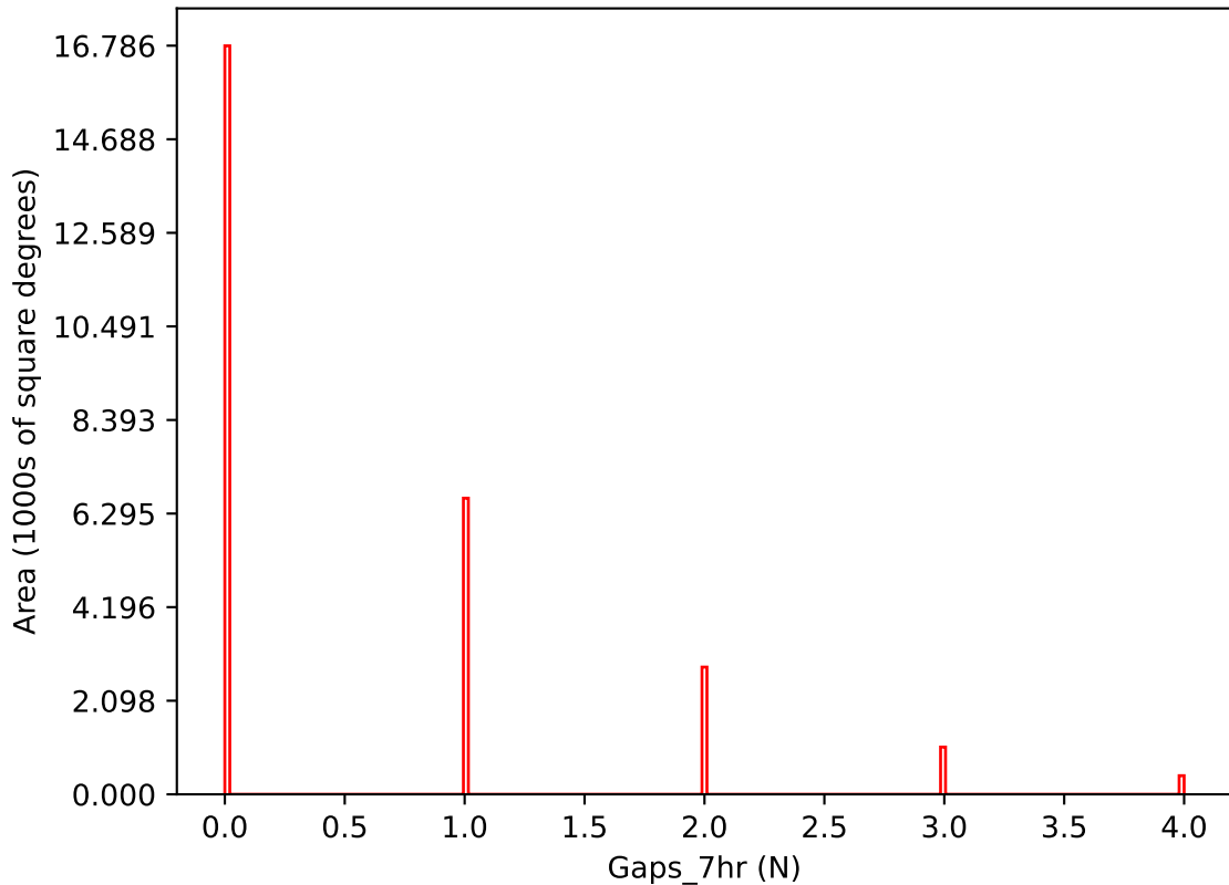
baseline_v3.4_10yrs i band: Gaps_7hr
