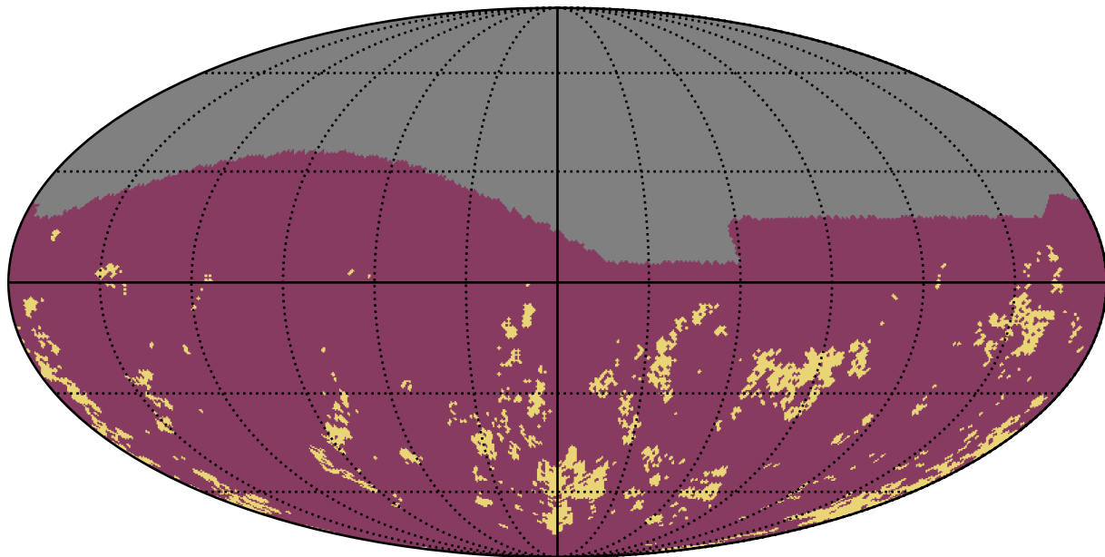
baseline_v3.4_10yrs g band: Gaps_7hr
