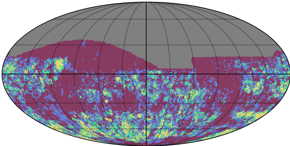
baseline_v3.4_10yrs z band: Gaps_3hr
