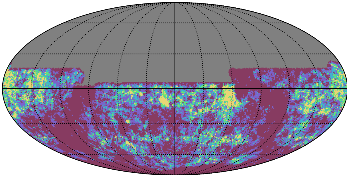
baseline_v3.4_10yrs y band: Gaps_3hr
