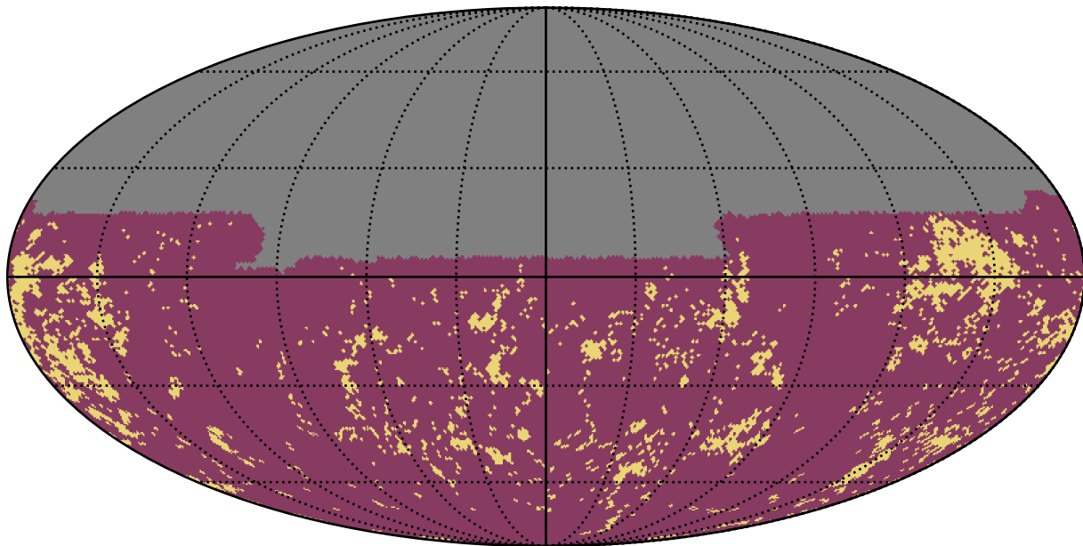
baseline_v3.4_10yrs u band: Gaps_3hr
