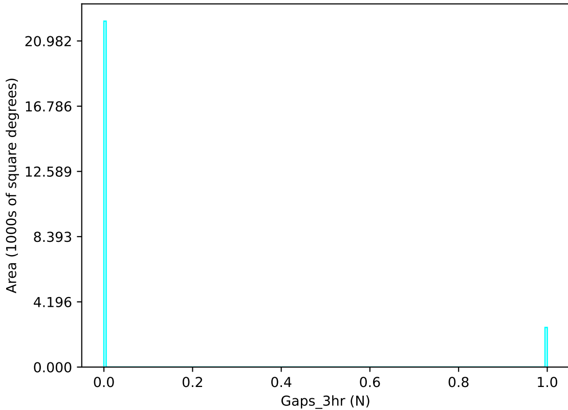
baseline_v3.4_10yrs u band: Gaps_3hr
