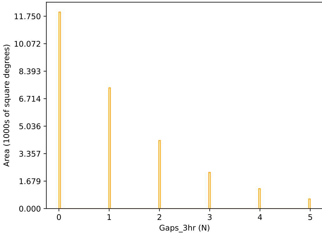
baseline_v3.4_10yrs r band: Gaps_3hr
