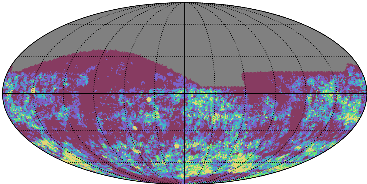
baseline_v3.4_10yrs i band: Gaps_3hr
