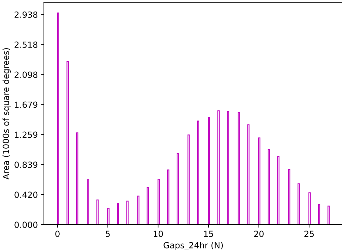
baseline_v3.4_10yrs z band: Gaps_24hr
