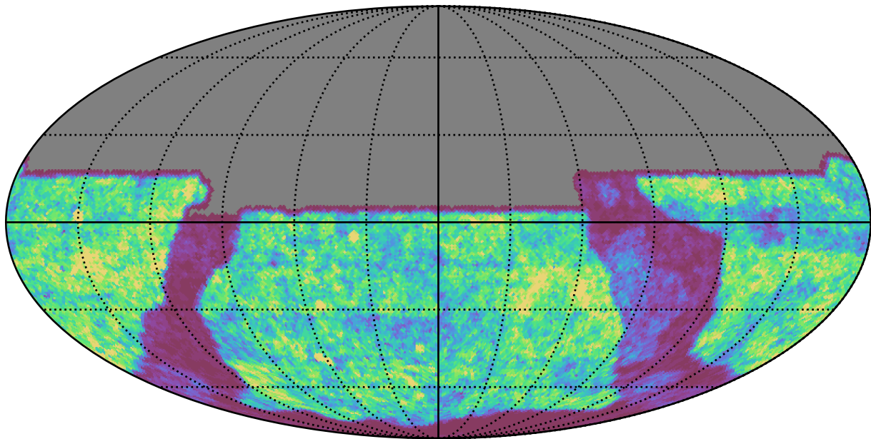
baseline_v3.4_10yrs y band: Gaps_24hr
