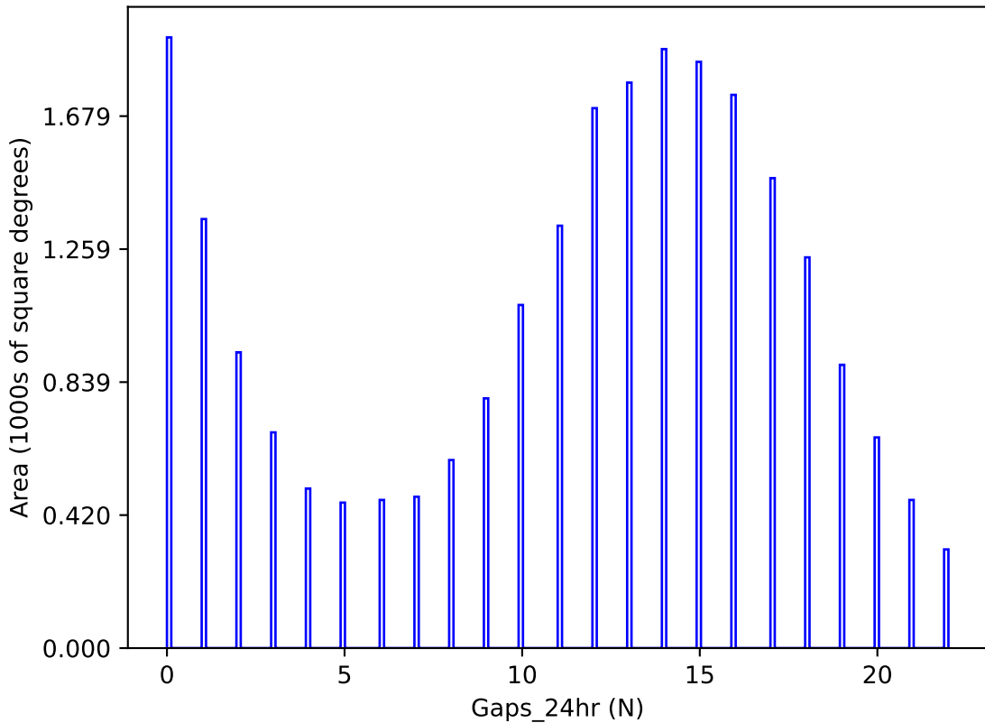
baseline_v3.4_10yrs y band: Gaps_24hr
