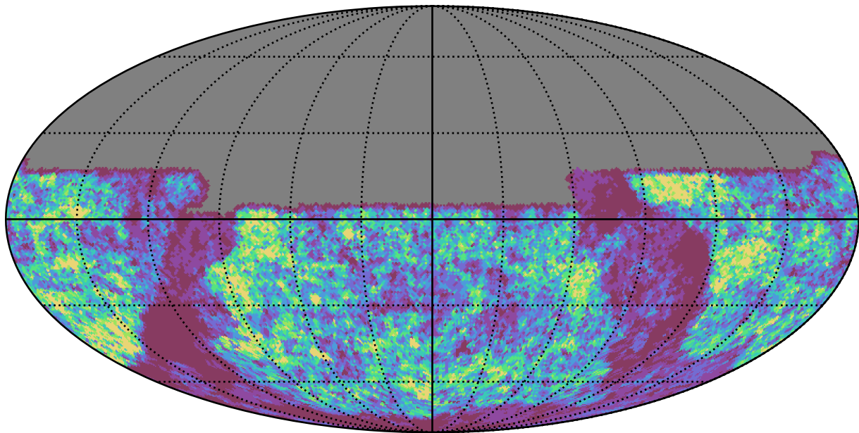
baseline_v3.4_10yrs u band: Gaps_24hr
