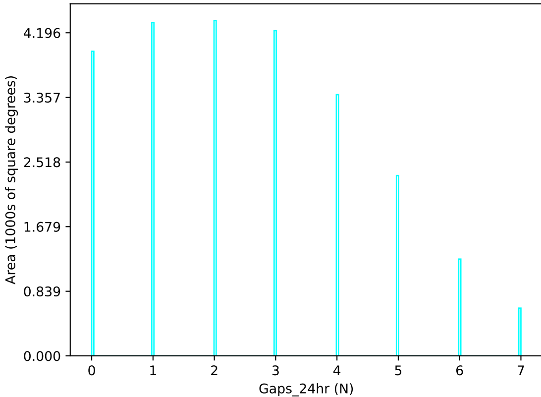
baseline_v3.4_10yrs u band: Gaps_24hr
