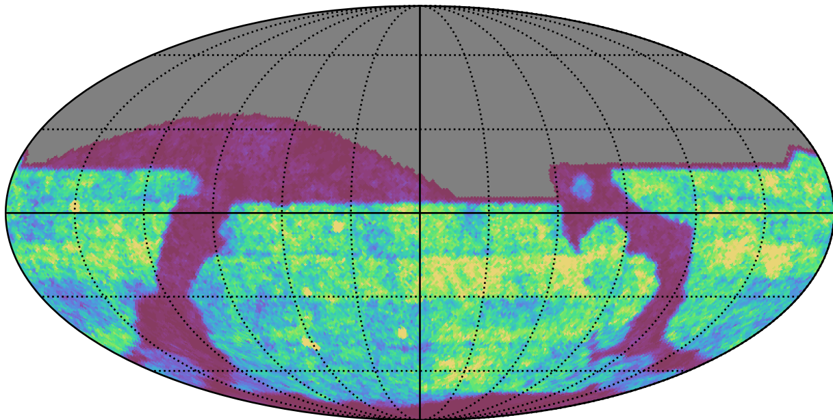
baseline_v3.4_10yrs r band: Gaps_24hr
