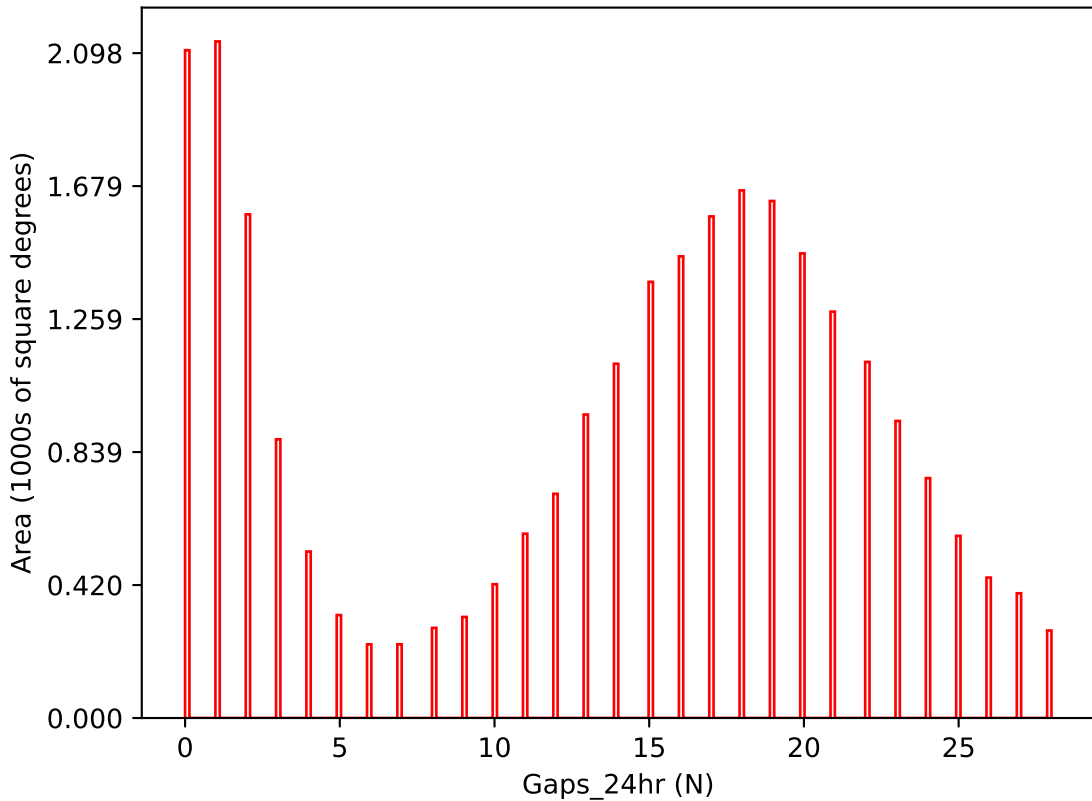
baseline_v3.4_10yrs i band: Gaps_24hr
